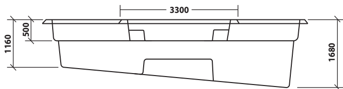
POOL SIDE ELEVATION WATER VOLUME = 17.8 KI.
