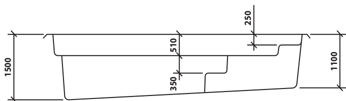
POOL SIDE ELEVATION
