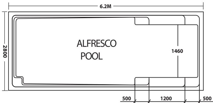
POOL PLAN LAYOUT
